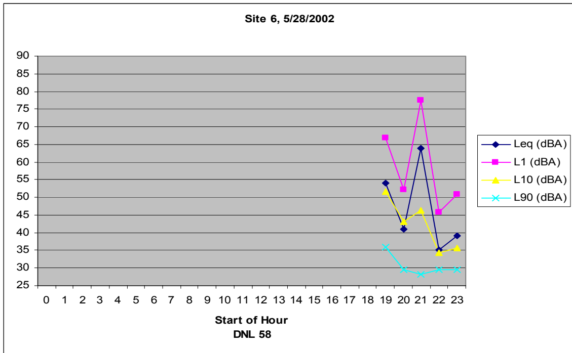
Figure B-3 Measured Hourly Noise Levels, Site 6
