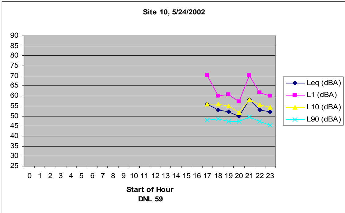
Figure B-6 Measured Hourly Noise Levels, Site 10
