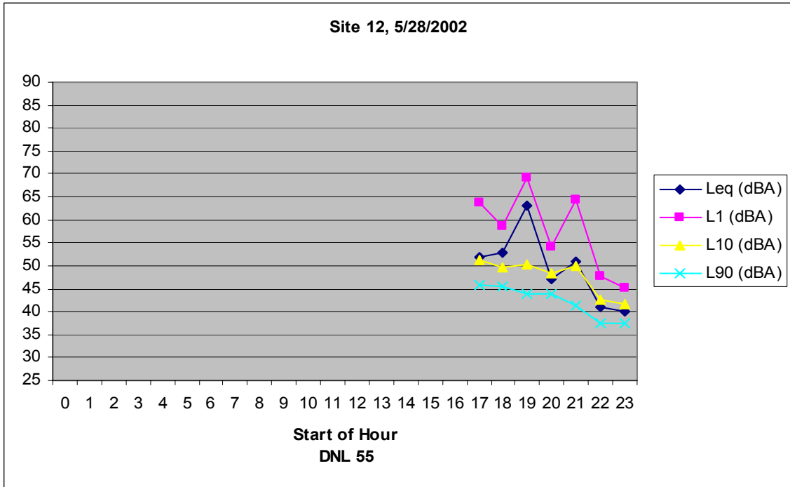
Figure B-7 Measured Hourly Noise Levels, Site 12
