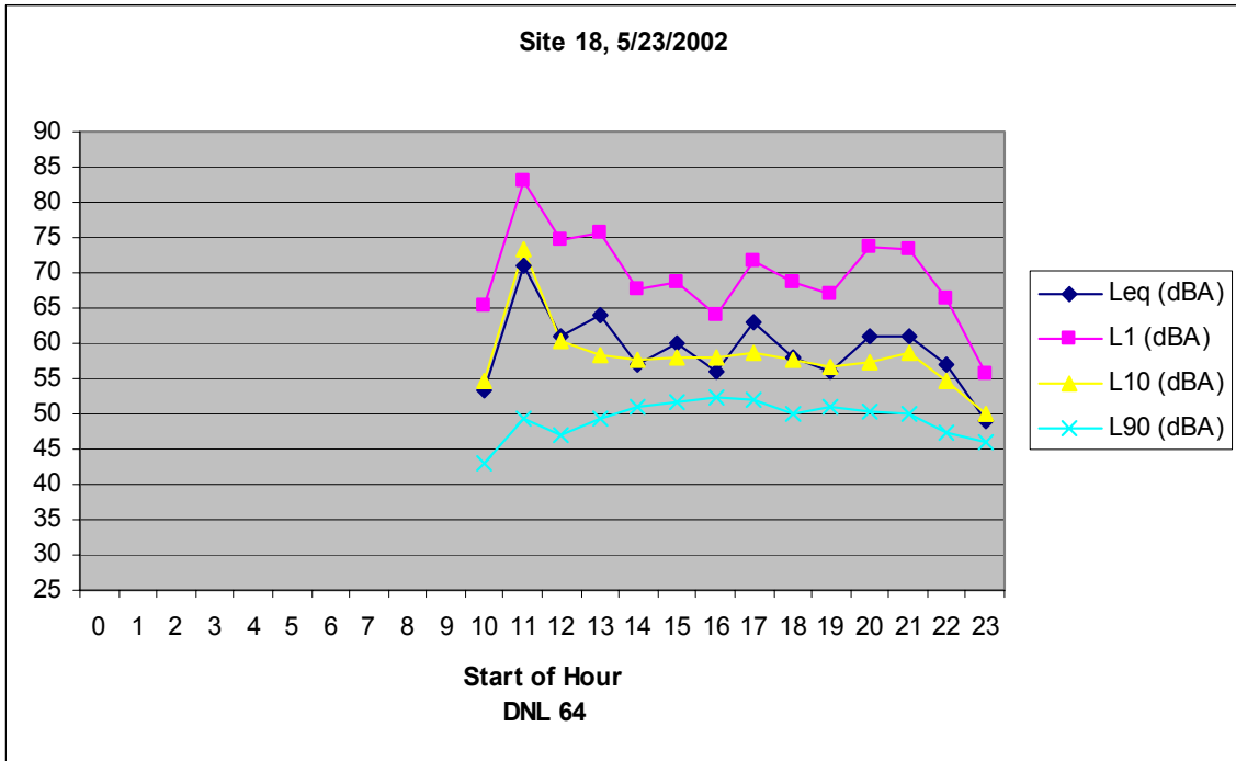
Figure B-9 Measured Hourly Noise Levels, Site 18
