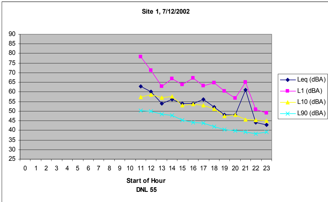
Figure B-1 Measured Hourly Noise Levels, Site 1
