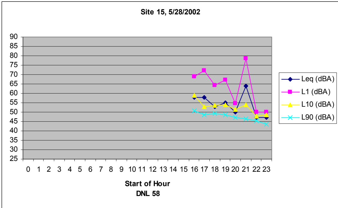
Figure B-8 Measured Hourly Noise Levels, Site 15
