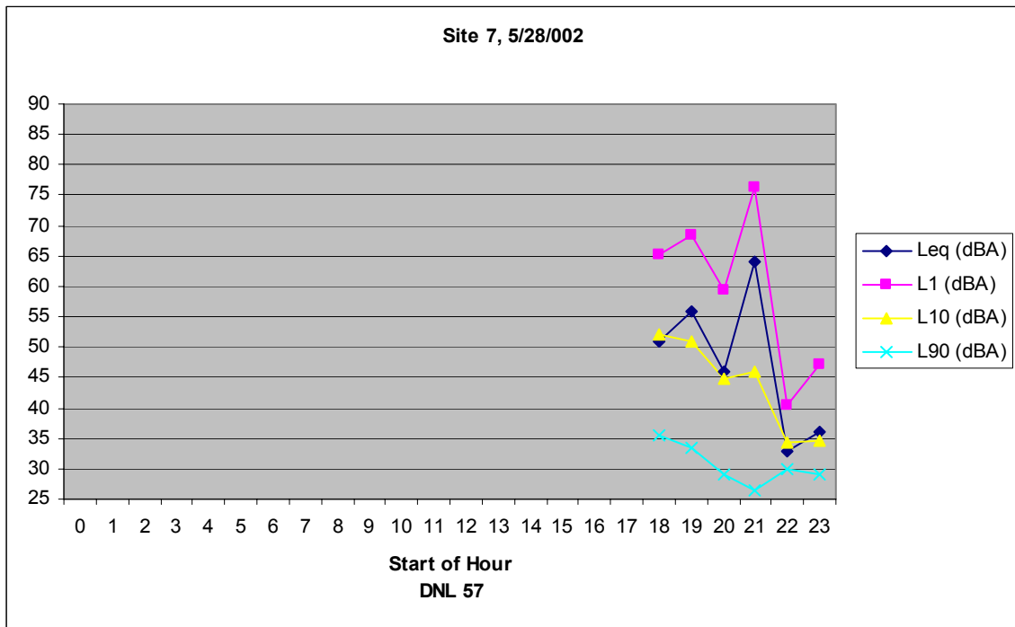
Figure B-4 Measured Hourly Noise Levels, Site 7
