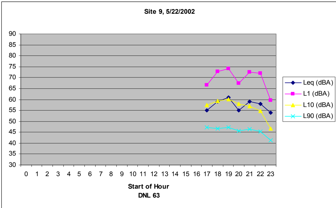
Figure B-5 Measured Hourly Noise Levels, Site 9
