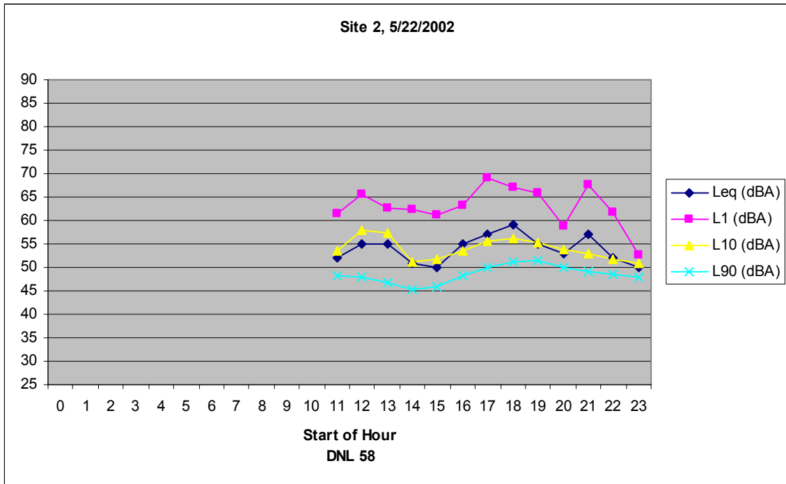
Figure B-2 Measured Hourly Noise Levels, Site 2
