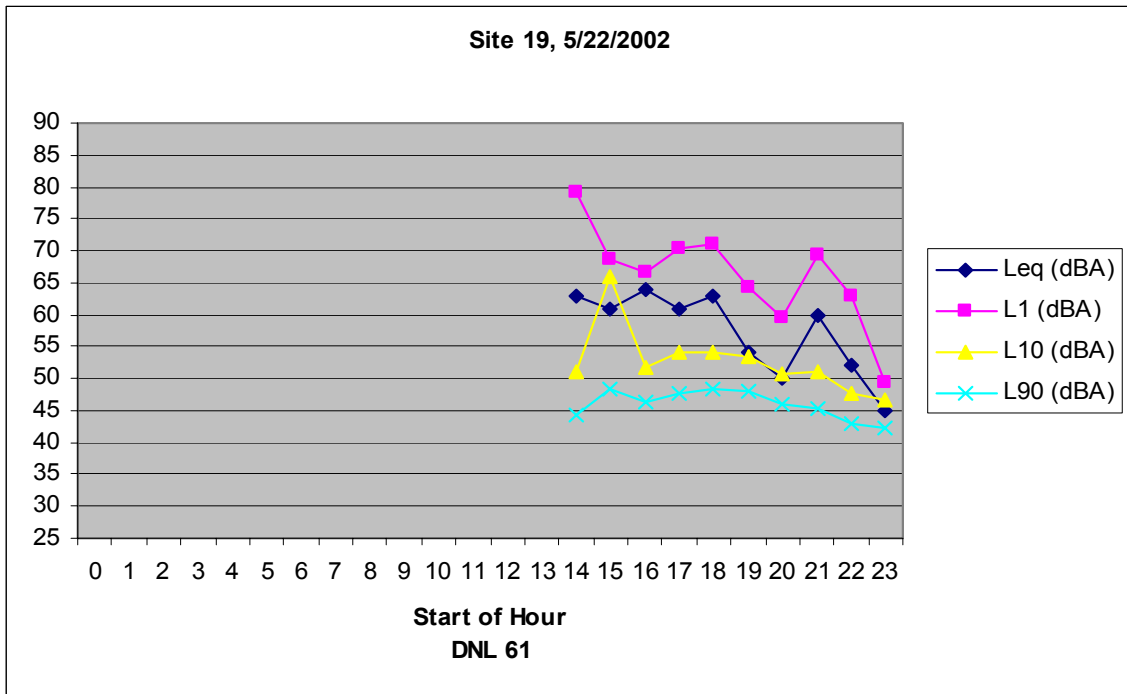
Figure B-10 Measured Hourly Noise Levels, Site 19
